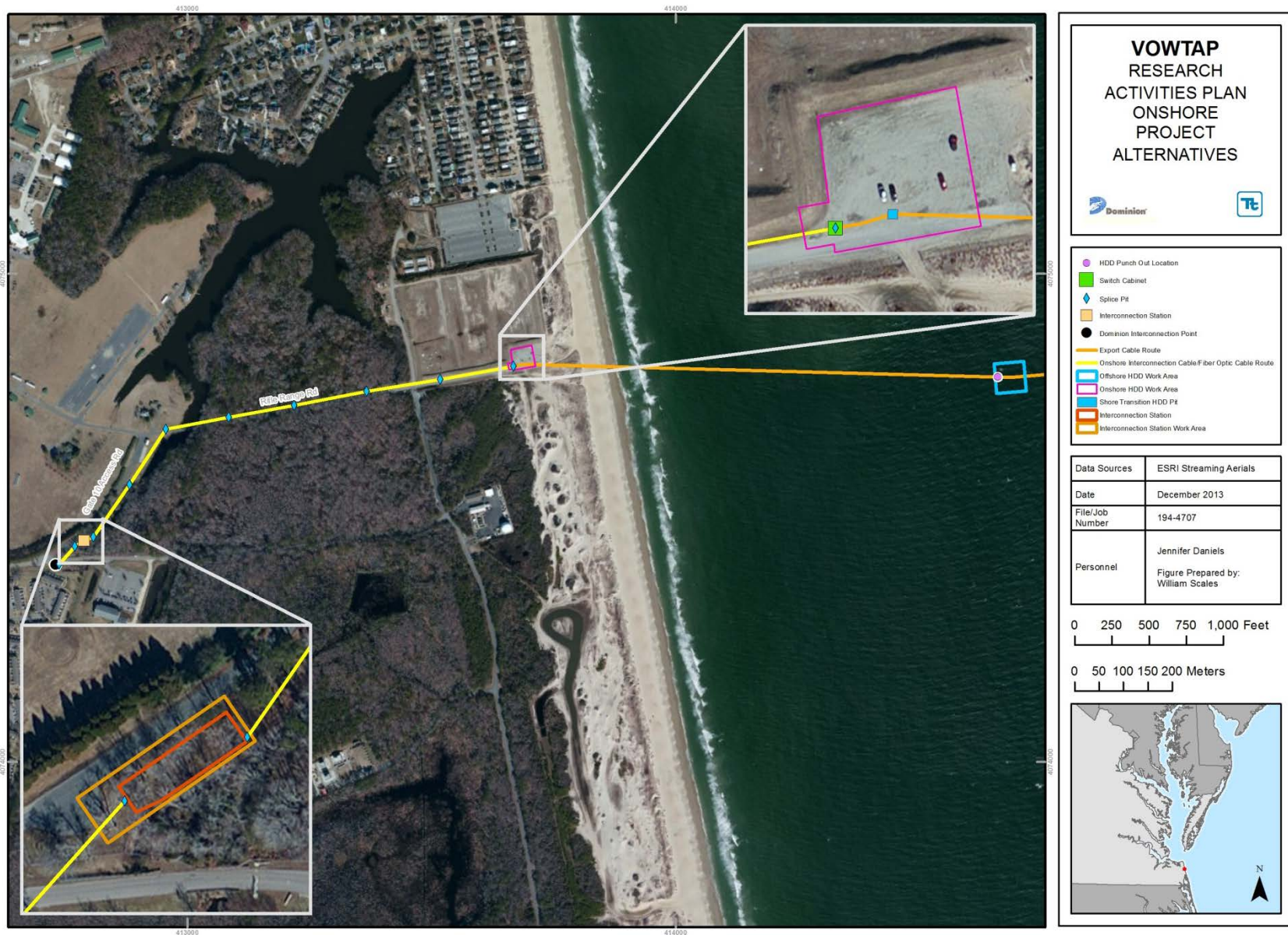
Figure 3.1-1. Onshore Project Facilities
